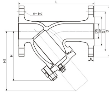
NPS ≥ 1 1/2 in
